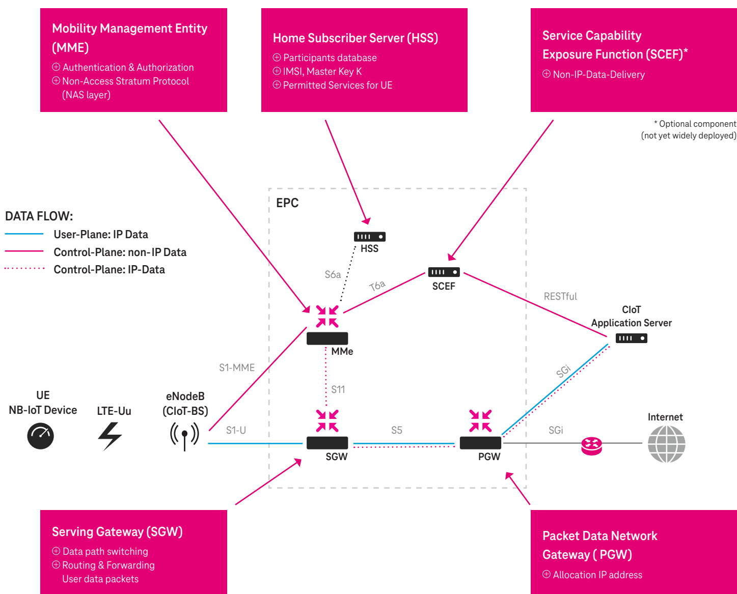
Figure 8: Evolved Packet System (EPS) for LTE/NB-IoT [26]
