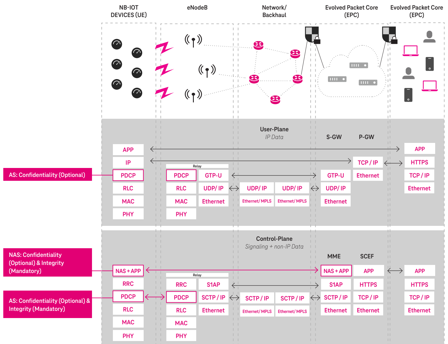
Figure 10: Protocol stack and security mechanism LTE/NB-IoT [26]
