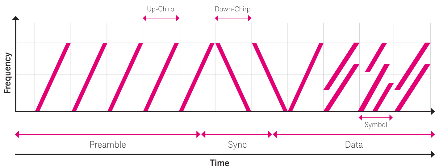
Figure 2: Chirp Spread Spectrum (CSS) modulation [14]
