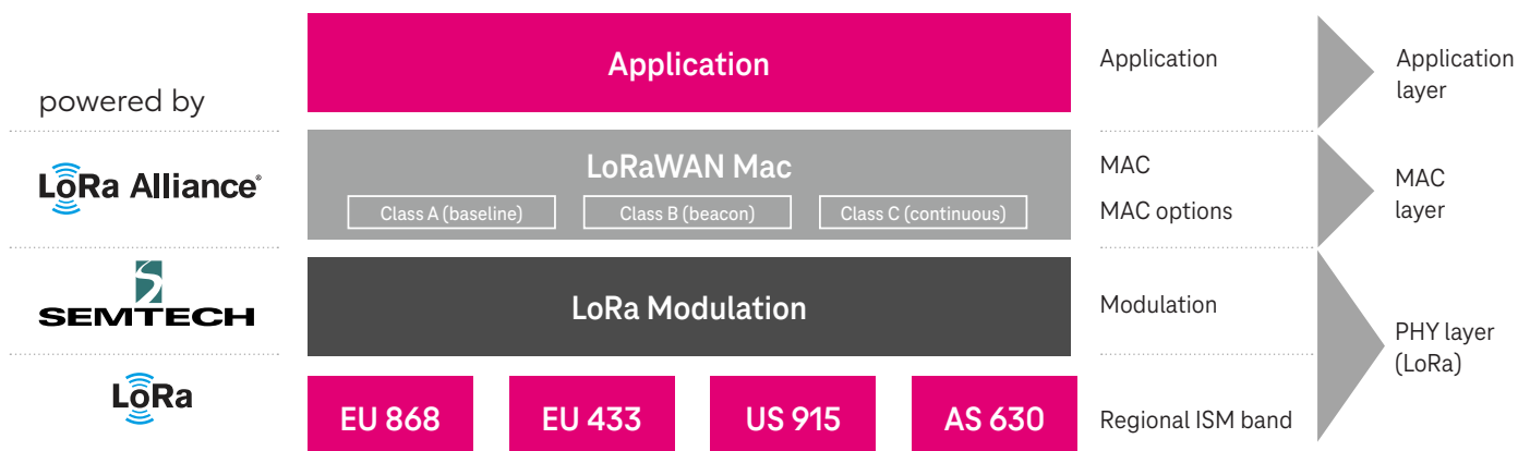
Figure 1: Layer structure and classification of LoRaWAN and LoRa [3]
