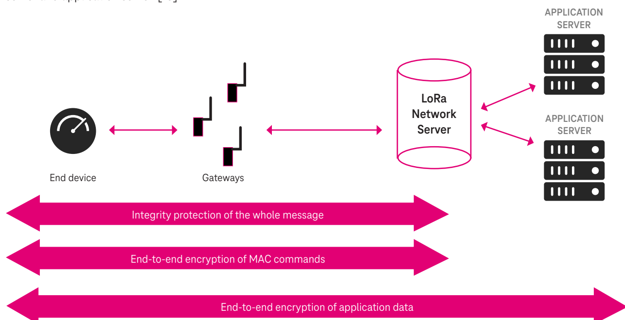
Figure 5: Security of LoRaWAN data messages
