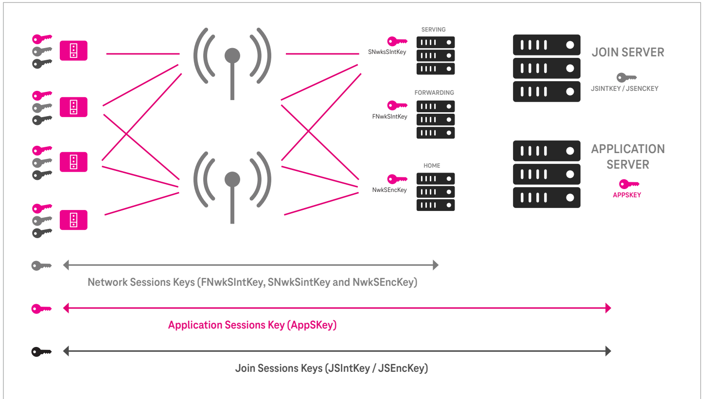
Figure 6: LoRaWAN architecture v1.1 (release 2017) [16]
